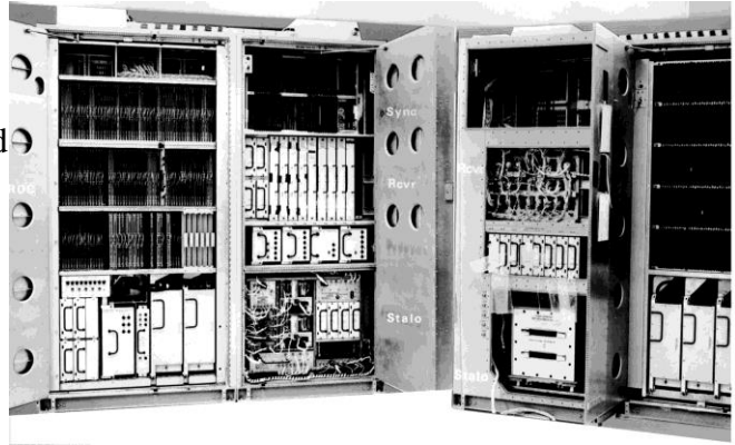
Fig. 9. DDT&E cabin equipment.
