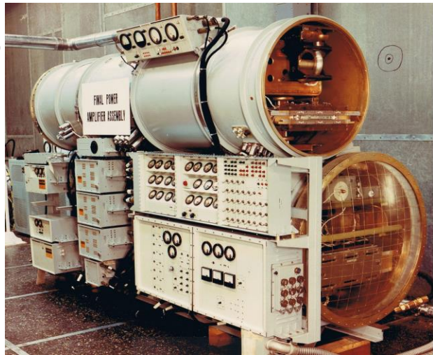
Fig. 6. Brassboard transmitter.
