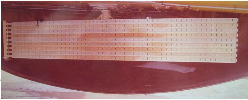
Fig. 3. ORT Antenna installed in EC-121 radome.
