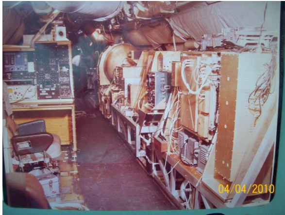
Fig. 4. ORT transmitter/receiver installed in EC-121 cabin.
