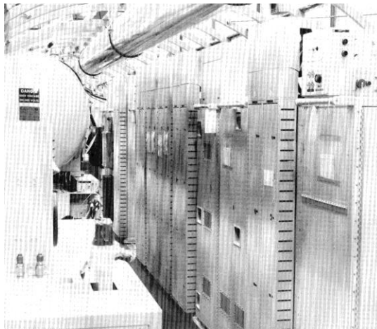
Fig. 7. Brassboard receiver.
